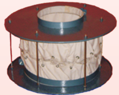
SMC 90240 POLISHING PAN For use with coating pan. Made of M.S. & provided with inner lining of superior canvas cloth, inner Dia 12x8" high with opening of 7" Dia neck
